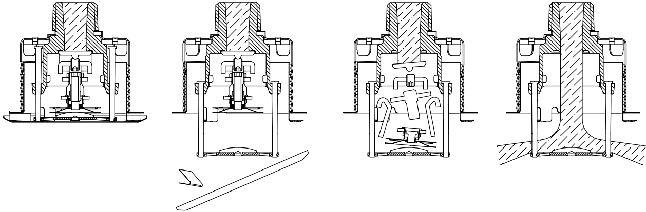
Normal Condition → Cover Plate Operation → Sprinkler Operation → Water Discharge Figure 2
